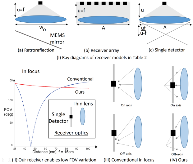
Figure 2: Our proposed design vs. other designs. In (I) we depict three common receiver designs, including retro-reflection (a), receiver array (b) and single detectors (c). Our design is a variant of (c), where we suggest a simple optical trick, such that the single detector is placed within the focal distance of the lens. This enables consistent FOV over range, as shown by the red curve in (II) and the designs in (III-IV). Simulations for a f = 15mm unit diameter lens.
